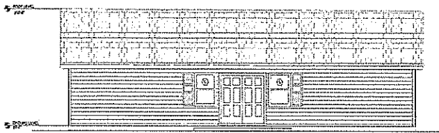
② EAST ELEVATION SCALE: 1/4" = 1'-0"
